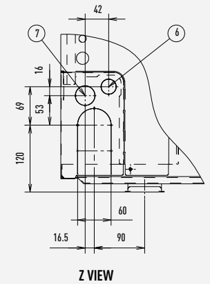
Z VIEW
