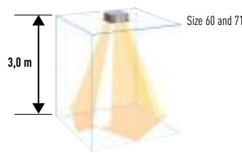
3-way discharge with the optional air-blocking materials
